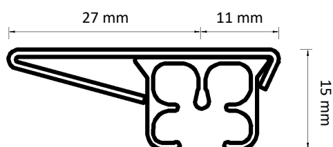
Ceiling Bracket
