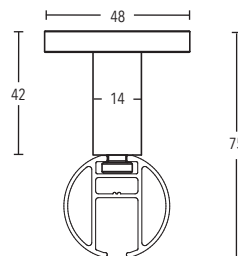
Ceiling bracket 42 mm art. no. 164942
