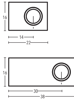
Café rod-wall bracket art. no. 21016-10-116 + 21018-10-116
