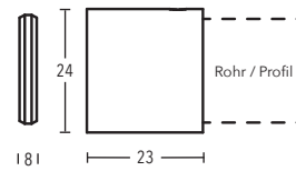
Recess bracket art. no. 207001
