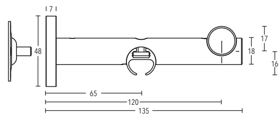
Combination-bracket art. no. 205220
