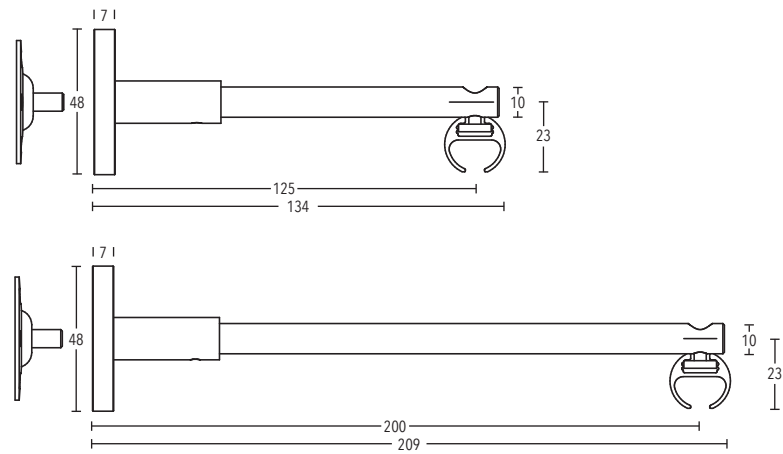
Wall bracket rail installation art. no. 284425 + 284500
