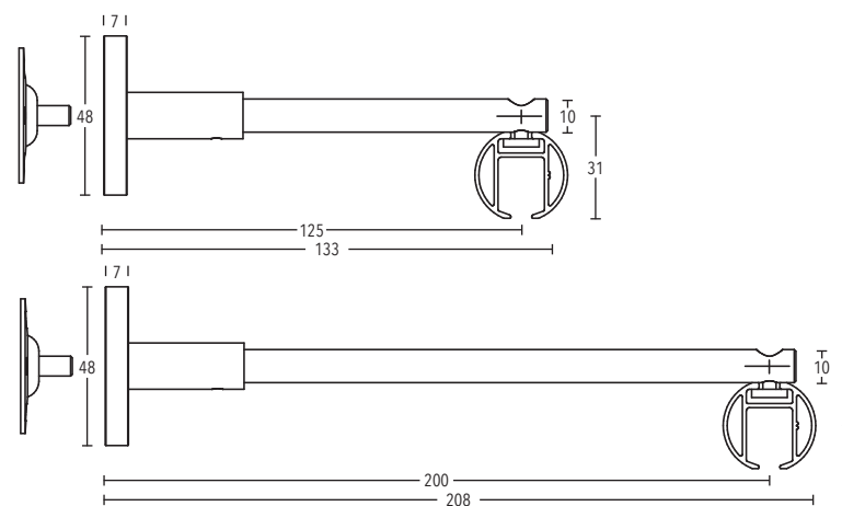
Wall bracket rail installation art. no. 284425 + 284500
