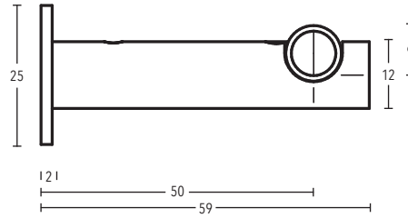
Café rod-wall bracket art. no. 21016-10-116 + 21018-10-116
