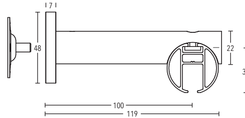
Wall bracket rail installation art. no. 354100
