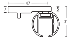
Snap-in Ceiling bracket 5 mm art. no. 11693-00
