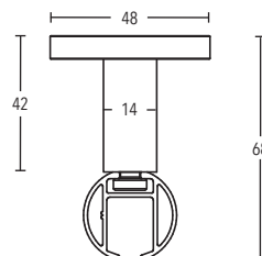
Ceiling bracket 42 mm art. no. 164942
