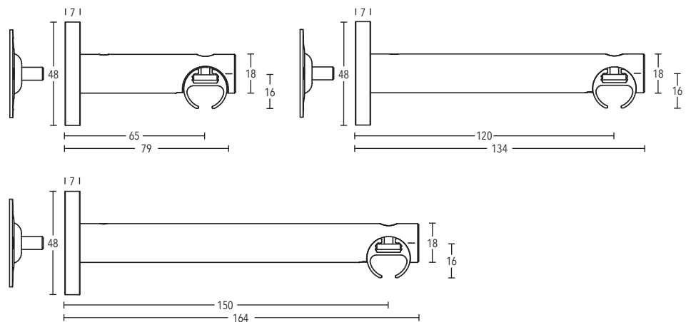
Wall bracket rail installation art. no. 204065 + 204120 + 214150
