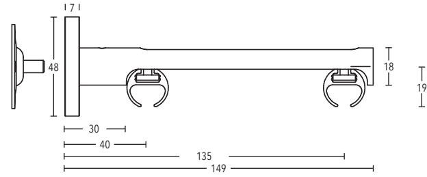
Multi-Wall bracket art. no. 205320
