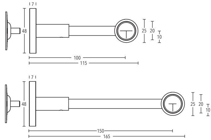
Wall bracket tube installation art. no. 204100 + 204150
