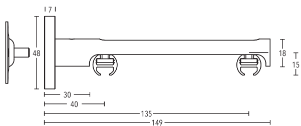
Multi-Wall bracket art. no. 205320-116
