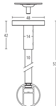
Ceiling bracket 500 mm art. no. 164995
