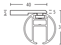
Ceiling bracket 3 mm art. no. 11592
