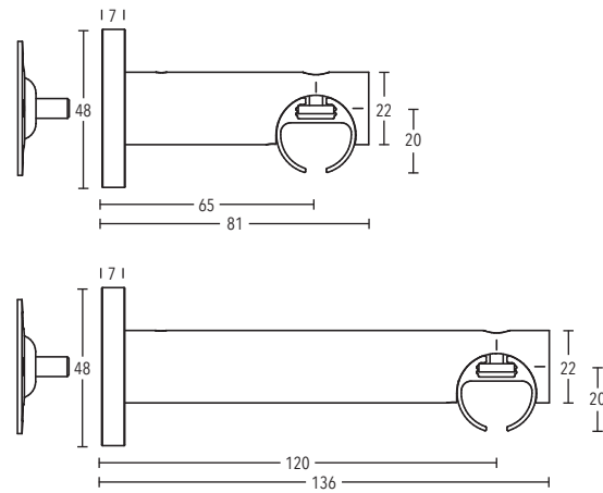
Wall bracket rail installation art. no. 244065 + 244120
