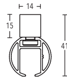
Ceiling bracket 15 mm art. no. 164915
