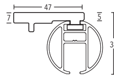
Snap-in Ceiling bracket 5 mm art. no. 11693-00
