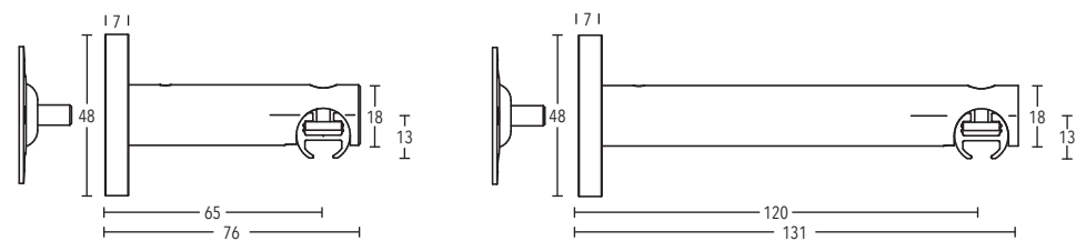
Wall bracket rail installation art. no. 164065 + 164120
