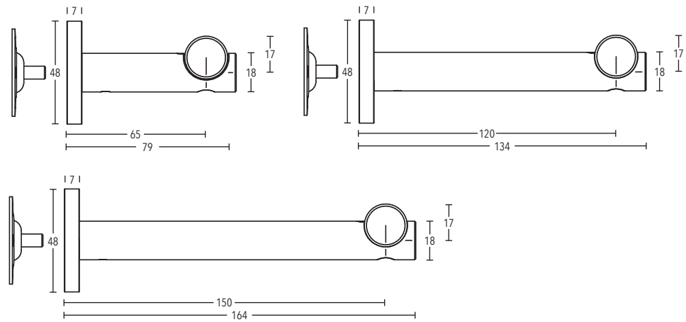
Wall bracket tube installation art. no. 204065 + 204120 + 214150 Please order cover art. no. 165001 separately
