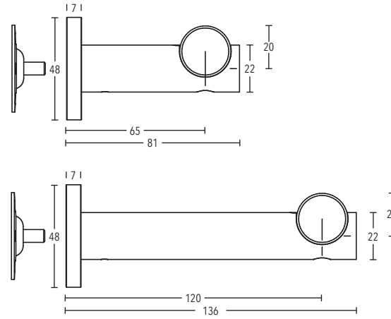
Wall bracket tube installation art. no. 244065 + 244120 Please order cover art. no. 165001 separately
