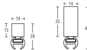
Ceiling bracket 15 mm + 35 mm art. no. 164915-116 + 164935-116
