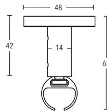
Ceiling bracket 42 mm art. no. 164942
