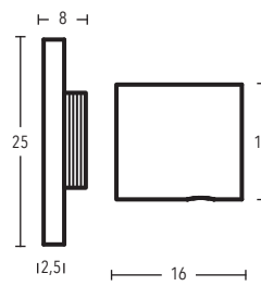
Recess bracket art. no. 107001-116
