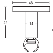
Ceiling bracket 42 mm art. no. 164942
