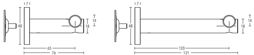
Wall bracket tube installation art. no. 164065 + 164120 Please order cover art. no. 165001 separately
