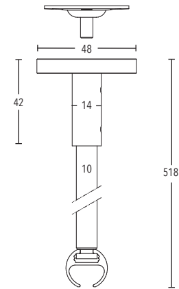
Ceiling bracket 500 mm art. no. 164995
