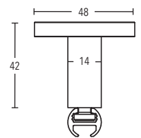
Ceiling bracket 42 mm art. no. 164942-116
