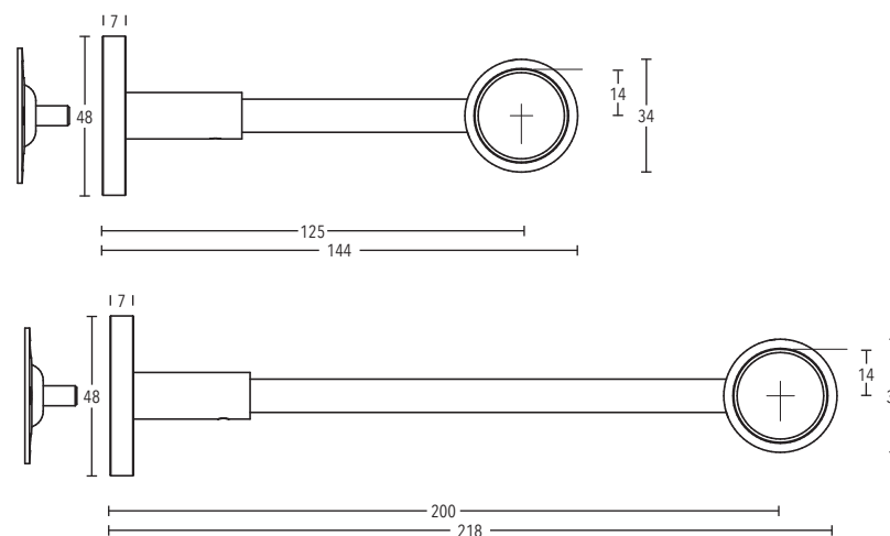
Wall bracket rail installation art. no. 284425 + 284500
