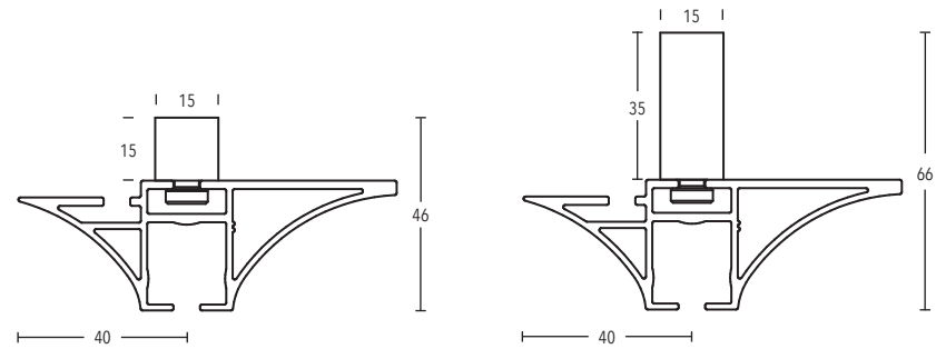
Ceiling bracket 15 mm + 35 mm art. no. 11473-15 + 11473-35
