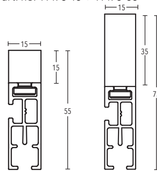
Ceiling bracket 15 mm + 35 mm art. no. 11473-15 + 11473-35
