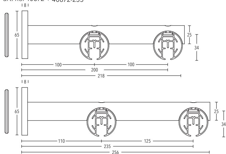
Wall bracket art. no. 40872 + 40872-235
