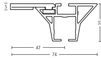
Ceiling bracket 3 mm Art.-No. 11592-00
