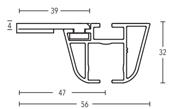
Ceiling bracket 3 mm art. no. 11592
