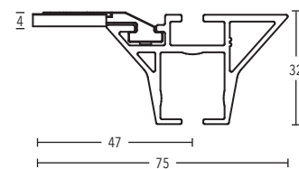
Ceiling bracket 3 mm art. no. 11597-00
