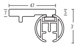
Snap-In ceiling bracket 6 mm art. no. 11693-00
