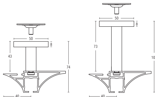
Ceiling bracket 43 mm + 73 mm art. no. 11473-50 + 11473-80
