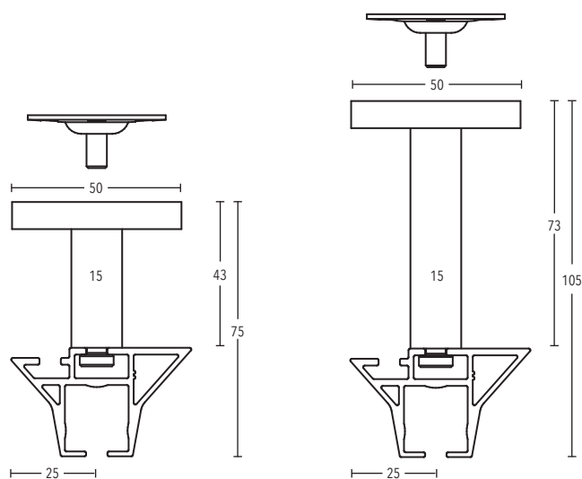
Ceiling bracket 43 mm + 73 mm art. no. 11473-50 + 11473-80
