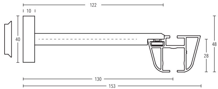
Wall bracket art. no. 11260-130
