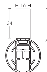
Ceiling bracket 34 mm art. no. 11873-30
