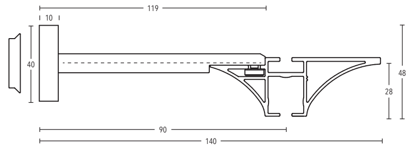
Wall bracket art. no. 11220-130
