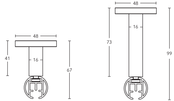
Ceiling bracket 41 mm + 73 mm art. no. 11873-50 + 11873-80
