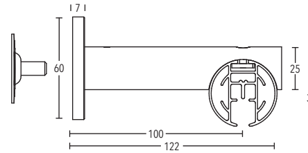
Wall bracket art. no. 40970
