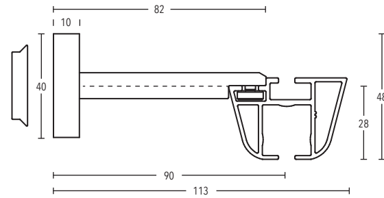
Wall bracket art. no. 11260-90
