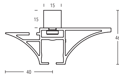
Ceiling bracket 15 mm art. no. 11473-100
