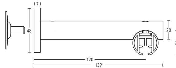
Wall bracket art. no. 11670-120
