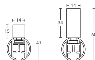
Ceiling bracket 15 mm + 34 mm art. no. 11873-15 + 11873-30
