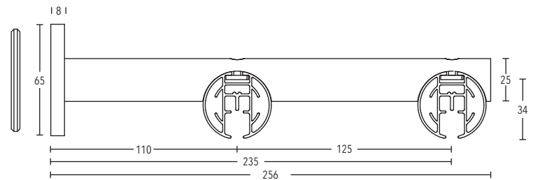
Wall bracket art. no. 40872-235
