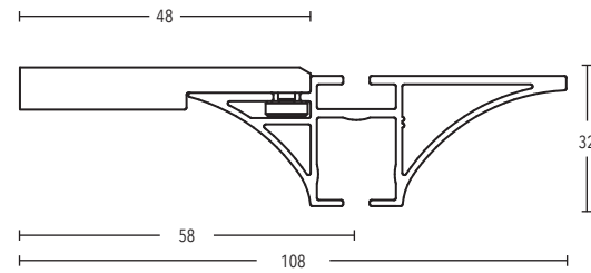
Ceiling bracket 5 mm art. no. 11220-20
