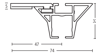
Ceiling bracket 3 mm art. no. 11592-00
