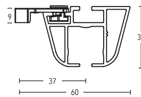
Clamping ceiling bracket art. no. 11590-10-00
