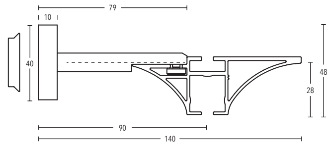
Wall bracket art. no. 11220-90
