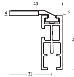
Ceiling bracket 3 mm art. no. 11597
