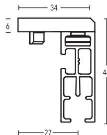
Ceiling bracket 6 mm art. no. 11590-1
