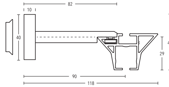
Wall bracket art. no. 11260-130
