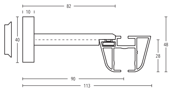
Wall bracket art. no. 11260-90
