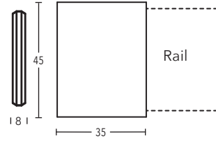
Recess bucket art. no. 122040
