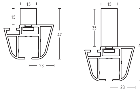
Ceiling bracket 15 mm + 35 mm art. no. 11473-15 + 11473-35
