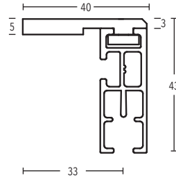
Ceiling bracket 3 mm art. no. 11592
