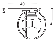
Ceiling bracket 3 mm art. no. 11592
