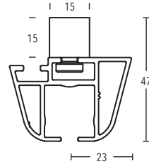
Ceiling bracket 15 mm art. no. 11473-100
