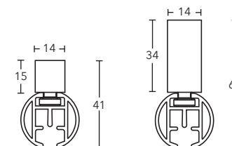
Ceiling bracket 15 mm + 34 mm art. no. 11873-15 + 11873-30
