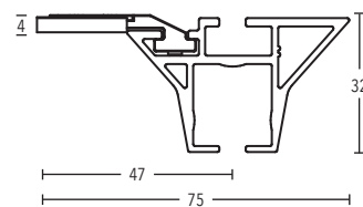
Ceiling bracket 3 mm Art.-No. 11597-00
