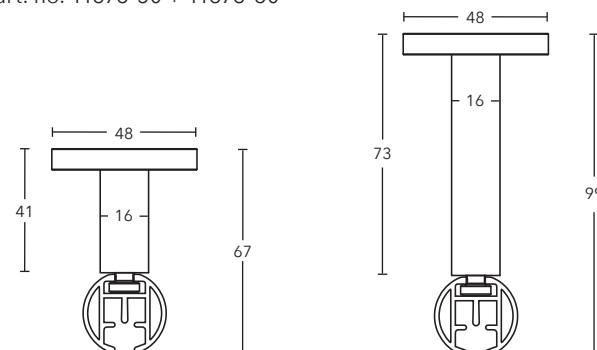
Ceiling bracket 41 mm + 73 mm art. no. 11873-50 + 11873-80
