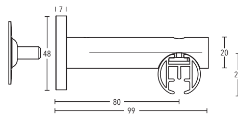
Wall bracket art. no. 11670 + 11670-120
