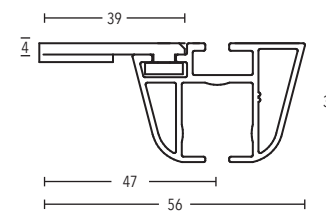
Ceiling bracket 3 mm art. no. 11592
