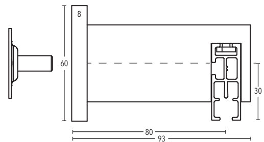
Wall bracket art. no. 11570-80
