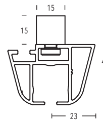
Ceiling bracket 15 mm + 35 mm art. no. 11473-15 + 11473-35
