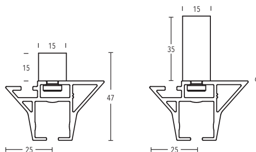
Ceiling bracket 15 mm + 35 mm art. no. 11473-15 + 11473-35
