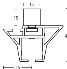
Ceiling bracket 15 mm art. no. 11473-100
