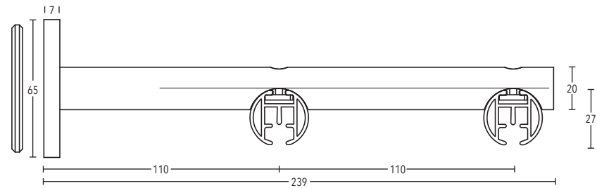
Wall bracket art. no. 11672-220
