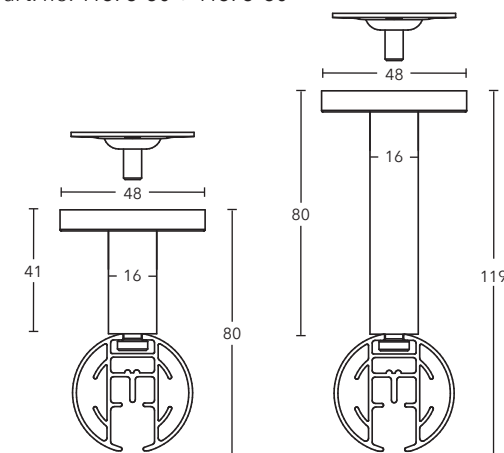
Ceiling bracket 41 mm + 80 mm art. no. 11873-50 + 11873-80
