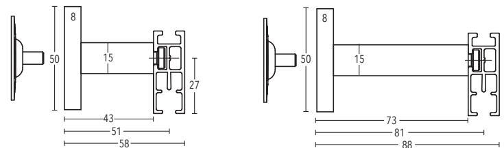
Wall bracket art. no. 11473-50 + 11473-80
