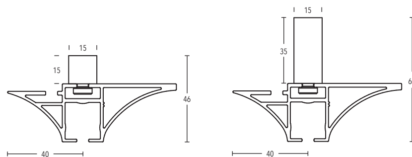
Ceiling bracket 15 mm + 35 mm art. no. 11473-15 + 11473-35
