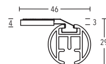
Ceiling bracket 3 mm art. no. 11597
